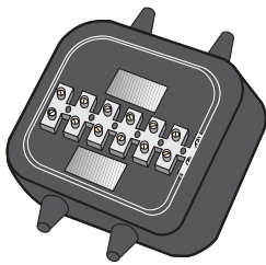
8 way junction box mounted in waterproof rubber base (Britax 3540.00)
