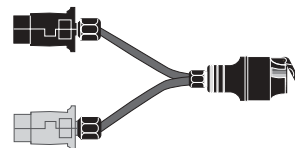
CONVERSION LEAD From 7 pin 12N & 12S to 13 pin With 200mm Cable
