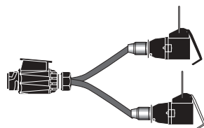
CONVERSION LEAD From 13 pin to 7 pin 12N and 12S With 200mm Cable
